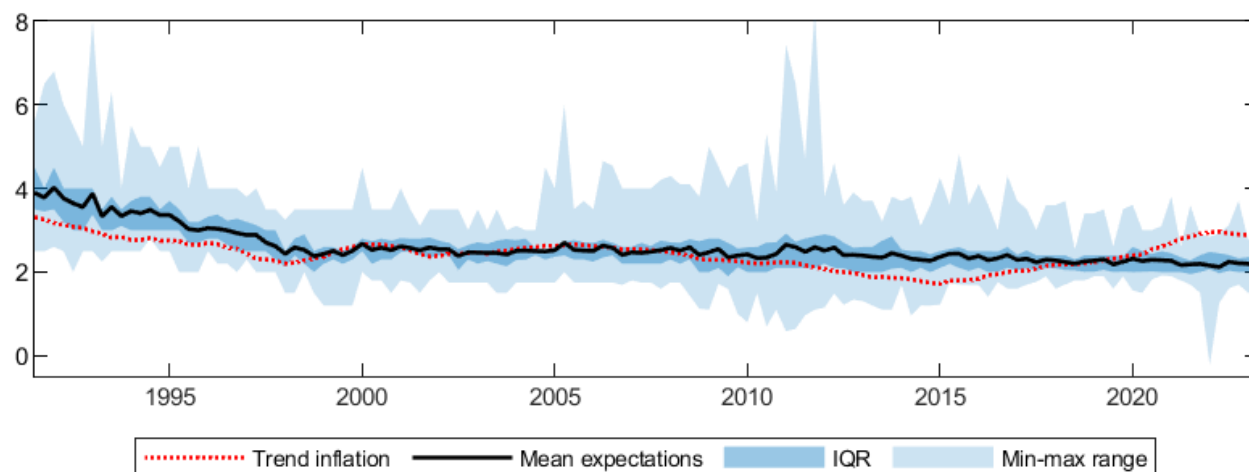
Figure 8: Trend inflation and full sample of long-run inflation expectations. Trend component of U.S. quarterly headline CPI inflation rate estimated using the trend-cycle model (red dotted line) and the mean (black solid line), the interquartile range (the dark blue bands), and the min-max range (the light blue bands) of the distribution of SPF long-run CPI inflation expectations including all forecasters in the survey.
